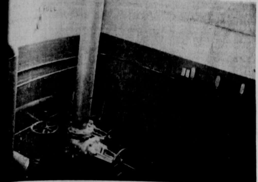
PLANT FLOODED —This pit at the power plant of the Community Public Service Co. was flooded. Pumps and pumps have been working all week to get the water out. The motors in this pit, which are used for the generators at the plant, were completely submerged, and will probably have to be replaced by plant superintendent Tom Waugh.
