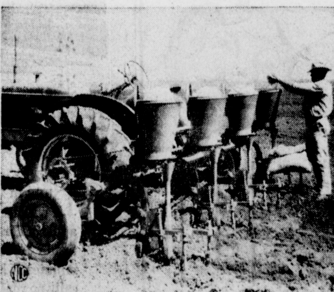
A cotton grower leads up the hoppers with seed in preparation for planting. With this tractor-drawn equipment, four rows can be planted simultaneously.
