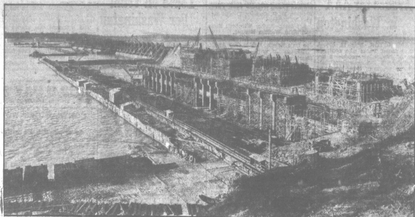
A giant barrier 6000 feet long and 65 feet high, the $38,000,000 Wheeler Dam, more than half completed, here stretches across the Tennessee river, one of the most important links in the TVA power program. Reared at the head of the lake formed by Wilson Dam, it is being built to relieve that structure at the time of peak loads. In the foreground are the foundation sections for the powerhouse. On the opposite side—the slab of white in the picture—is the navigation lock which army engineers built before TVA took over construction. Wheeler Dam, midway between Florence and Decatur, Ala., will create a reservoir of about 100 square miles.
