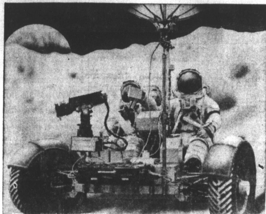
LUNAR ROVING VEHICLE: The Apollo 15 astronauts will take with them to surface of the Moon a four-wheeled vehicle that will be used to transport themselves and equipment over the Lunar surface. The "Rover" has a capacity of 970 pounds with both astronauts comfortably seated with safety seat belts. Traveling at top speed of 10 miles per hour the spacemen will be equipped to cover much more area than in previous Apollo landings.
