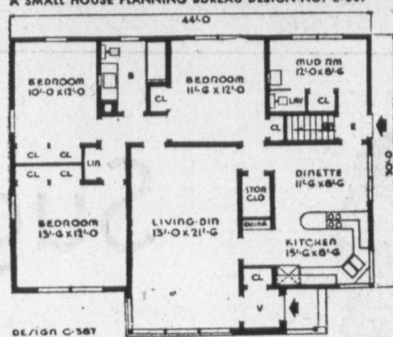
A SMALL HOUSE PLANNING BUREAU DESIGN NO. C-387
