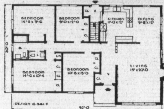
A SMALL HOUSE PLANNING BUREAU DESIGN NO. C-381-F
