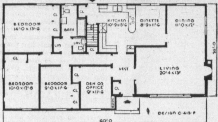
A SMALL HOUSE PLANNING BUREAU DESIGN NO. C-415-F
