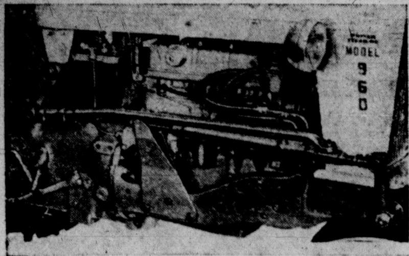
STEERING UNIT —Power steering on new Ford tractors is accomplished, as shown here, by a linkage type unit that does not interfere with mounting the tractor.
