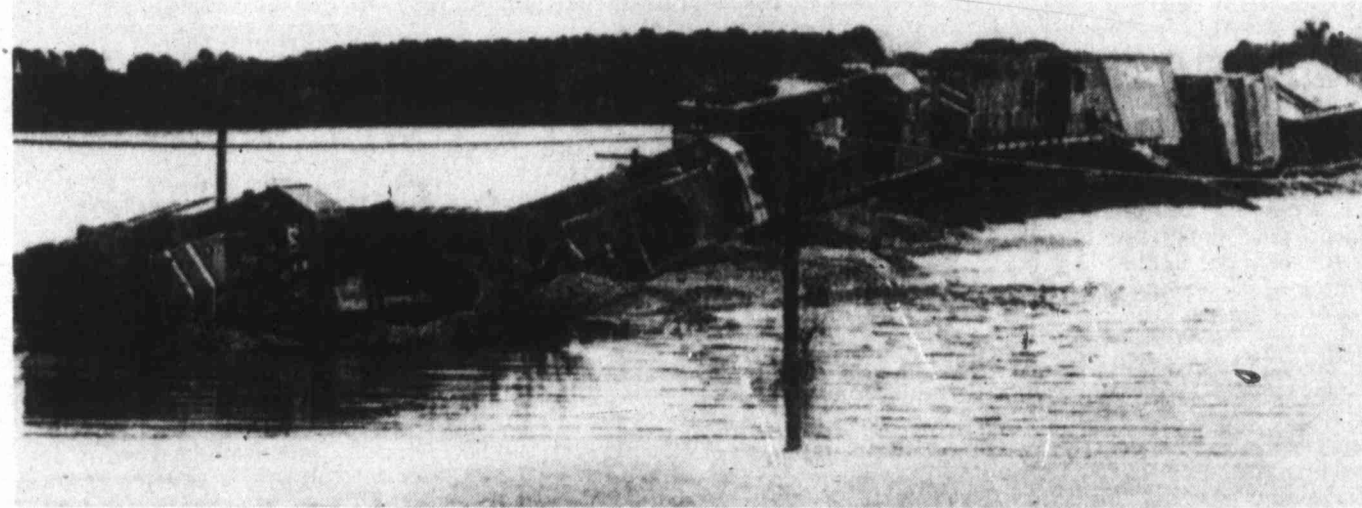
FREIGHT TRAIN DERAILED BY FLOOD WATERS — Floodwaters from heavy thunderstorms washed out a track embankment along Hickory Creek south of
