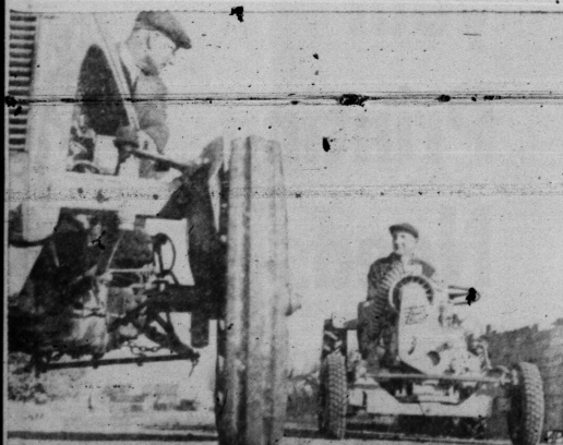
COMPACT TRACTOR —"Mini Clarker," tiny tractor—only 36 inches high—dwarfed by rear wheel of conventional farm tractor. Its designer says it can pull two tons with ease, and that its 19-horsepower engine will run all day on two gallons of fuel.
