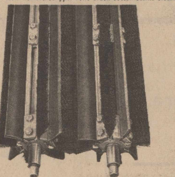
New flexible stripper rolls brush cotton stalks clean.
