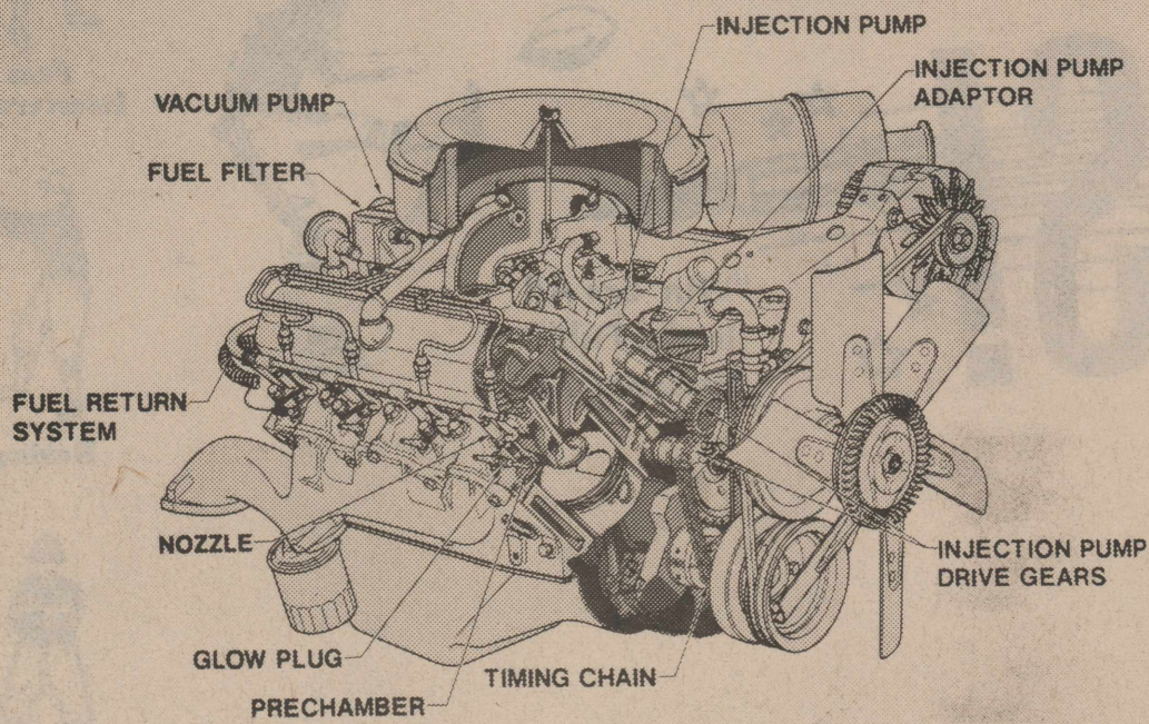
1978 General Motors Diesel Engine Cutaway
