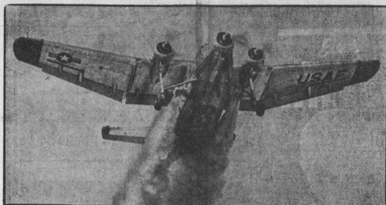
NEWEST LIGHT TRANSPORT —Six jet rocket units and three engines enable the U. S. Air Force's newest light assault transport to take off in a space of less than 500 feet. Weighing 20 tons, the Northrop Raider C-125 was designed to transport heavy loads in and out of small, unimproved clearings. The photograph was made during one of the ship's test flights at Hawthorne, Calif.
