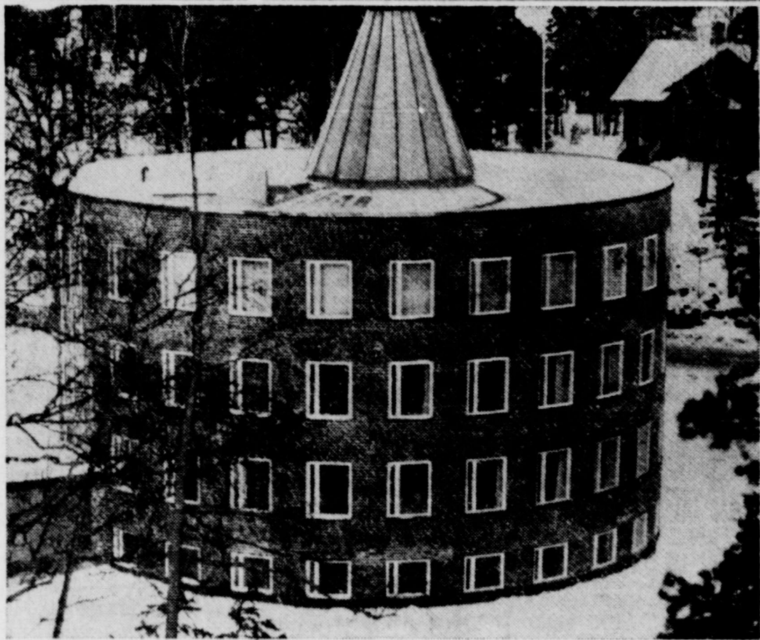
A ROUND CITY HALL—This is the unique round Municipal Hall of Gustafsberg, a suburb of Stockholm, Sweden. The roof is removable, permitting the construction of new floors when they are needed. Rooms stretch out in the shape of fans from the central staircase and are partitioned by movable walls. The "lantern" on the roof resembles a lighthouse.
