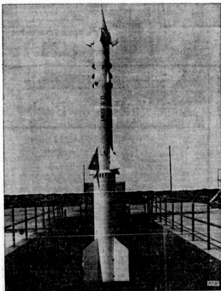
U. S. ARMY'S NIKE ZEUS anti-missile missile has a new look. The new configuration has shorter, more blunt control surfaces replacing triangular fins near the nose of the missile. During a recent test firing at White Sands Missile Range, N. M., the new fins resulted in a considerable increase in performance of the Zeus. Western Electric Company is prime contractor for the Zeus system. Bell Telephone Laboratories has design and development responsibilities and Douglas Aircraft builds the missile.
