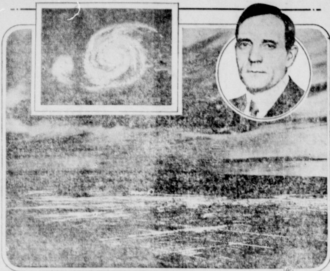
Dr. Edwin Hubble (upper right) explains that measurement of distance of far-away ob- jects is like viewing lights of Los Angeles and surrounding towns (below)—and from them alone trying to tell what kind of people live there. Upper left shows a spiral nebula as viewed through the 100-inch telescope.
