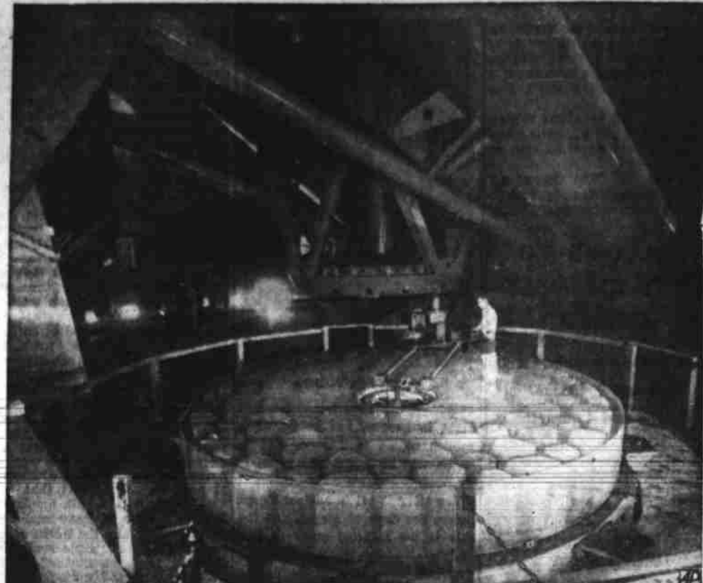
POLISHING JOB — Don Hendrix, Mt. Wilson Observatory optician, operates a special machine to remove 20 millionths of an inch from part of the surface of the 200-inch mirror for the Hale telescope on California's Palomar Mountain.
