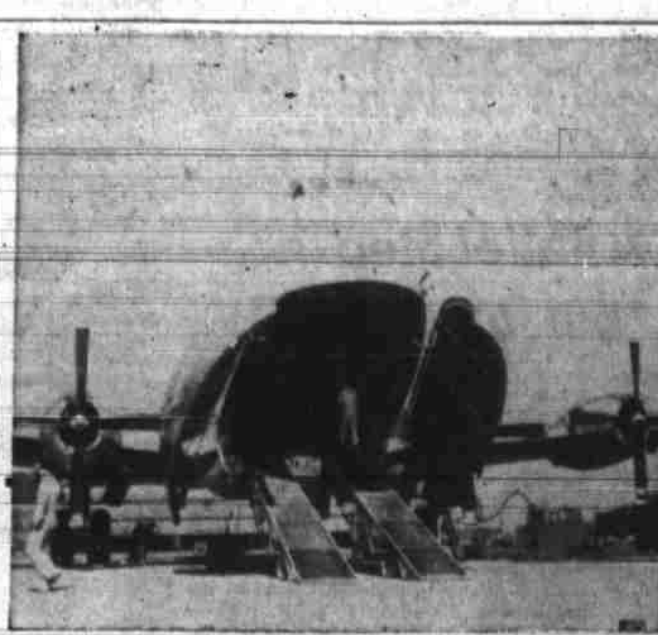
TRUCKS CAN BE DRIVEN INTO NEW CARGO CARRIER — Tanks, field guns, bulldozers and fully loaded trucks can be driven up this loading ramp into the Air Force's new troop and cargo transport, the Douglas C-124 "Globemaster II." The clamshell doors provide this loading hatch in the nose of the Air Force's largest production transport which was built at the Douglas plant at Long Beach, Calif. Loading of static cargo is facilitated by an electrically operated elevator which can be lowered from the center of the cargo section. (AP Wirephoto from Department of Defense).
