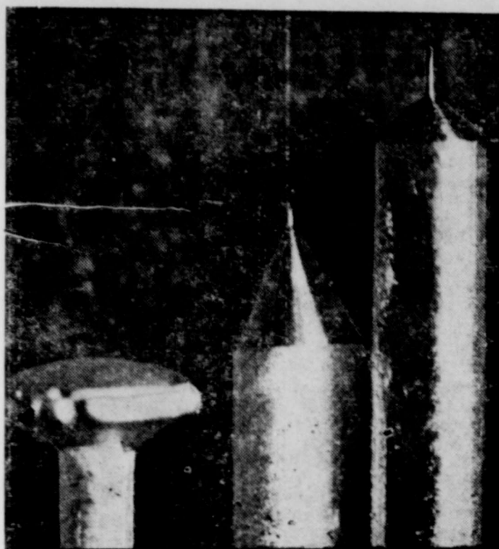
GIANTS' TOOLS —That's what the huge spike, at left, and the mammoth drills appear to be. Actually, the "spike" is the head of a pin, and the tiny points of the drills are as small as .001 inch in diameter. They have been used under the microscope at General Electric's Schenectady, N. Y., laboratories to perforate a human hair, and find use in making of ultraprecise equipment.
