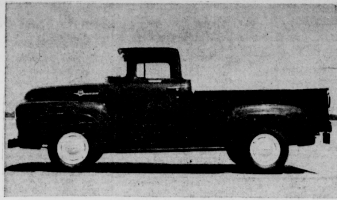
NEW CAB STYLE —Ford's F-100 pickup truck with wraparound windshield and hooded roof is available in a 110 or 118 inch wheelbase to carry either a 45 or 65 cubic foot box. Powered by a 223 cu. in. 1-block six cylinder engine rated at 133 hp, or a 272 cu. in. V-8 rated at 167 hp, the pickup has five transmissions available: standard, overdrive, Fordomatic and heavy duty 3 speed and 4 speed. Ford's 1956 trucks go on display at 6,800 Ford dealer showrooms September 23.
