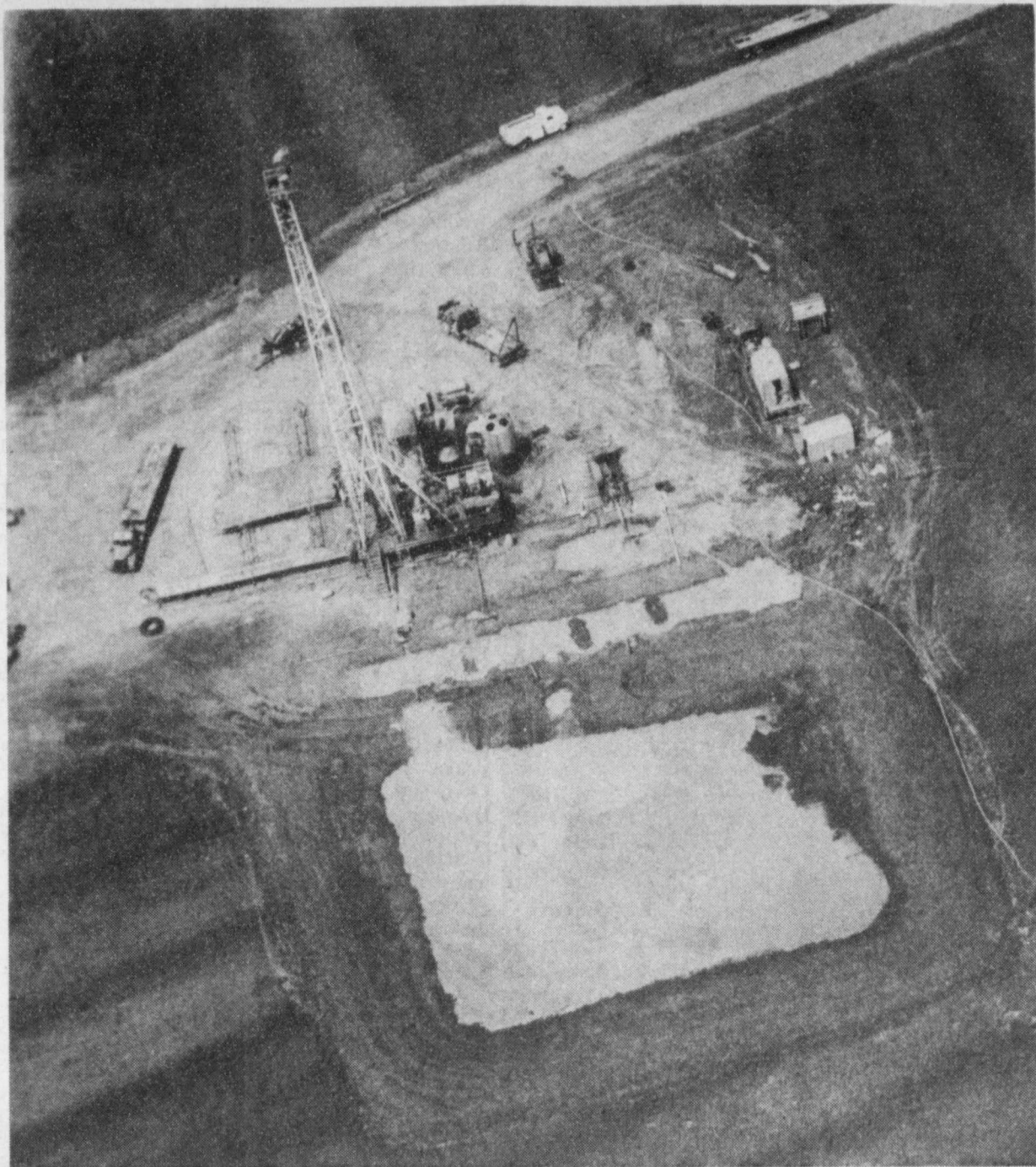
OIL WELL Drilling is in active progress in Red River County. Westbrook Drilling is working on the Ford No. 3 Well, and expects to be finished with it soon. (Staff Photo)
