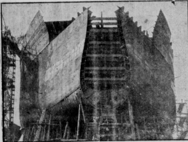
FROM THE SUEZ CRISIS: SWIFT COMPLETION—The 55,000-ton American oil tanker "Minneoma" nears completion at the shipyard in Dunkerque, France. Possible closure of the Suez Canal has speeded work at Dunkerque on super tankers of 100,000 tons—capable of sailing economically around the tip of Africa.
