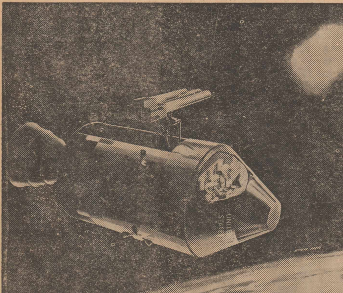
A LOOK AT THE SUN. When the earth-orbiting Apollo manned missions are launched, one of the duties of the U.S. astronauts will be to photograph the sun through large astronomical telescope mounted on their space vehicle. In space, the sun can be observed free of most atmospheric distortions. — WFS Photo
