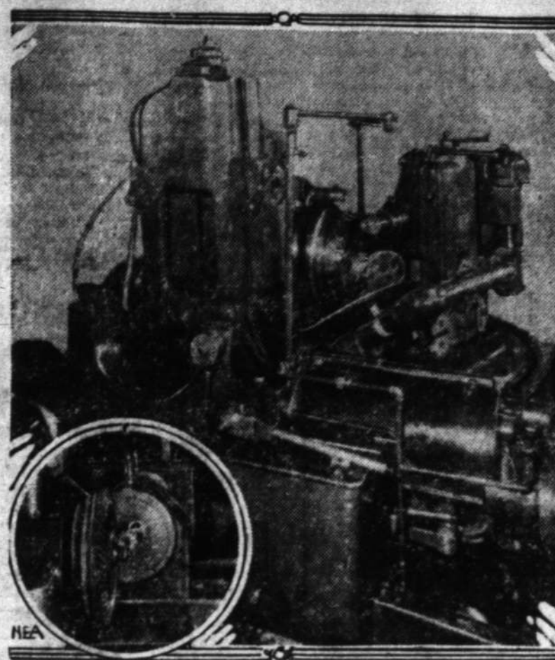
Swinging in, out and around, this machine cuts the teeth of an entire gear without the aid of man. Inset shows a set of gears on test in the silent room.
