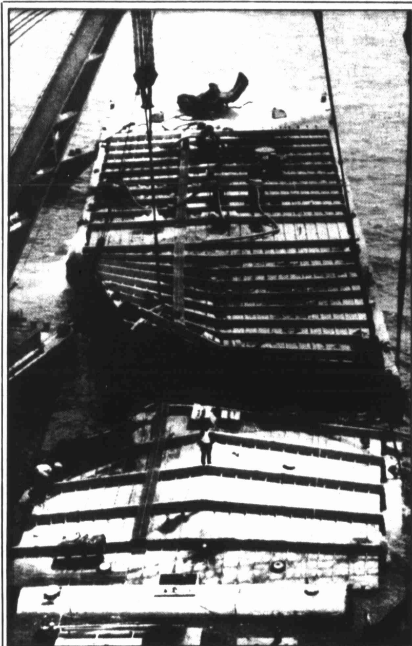
HOUSTON — Salvage crews Wednesday cut the crippled oil barge for shipment to a scrap yard. The gash on the left is where the barge was hit by the ship in the Houston ship channel, causing a massive oil spill in Galveston Bay.
