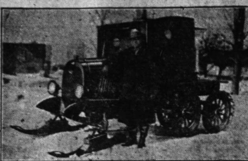
Converting a Chevrolet car into a Snowmobile mounted on skis and tractor wheels has solved winter transportation problems for Charles Survell of Newberry, Mich.
