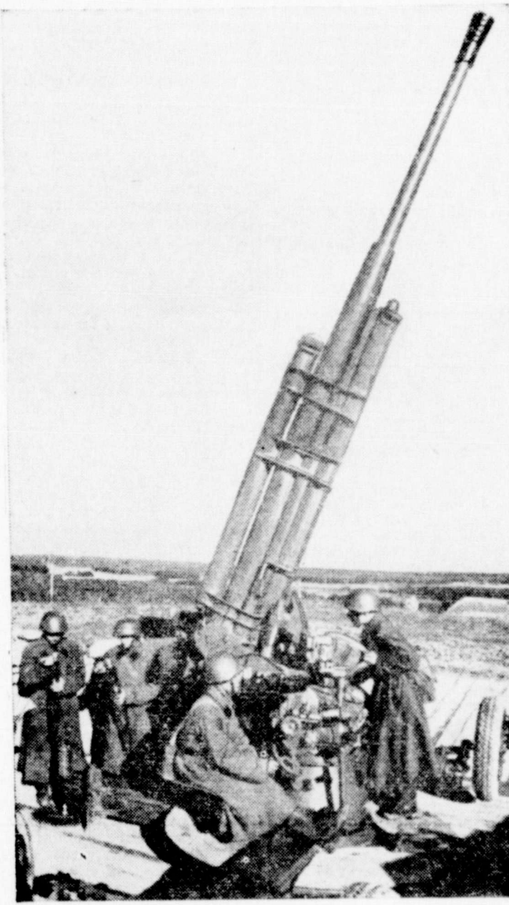
ANTI-AXIS—A crack Soviet crew mans a Zenith anti-aircraft gun which has helped to effectively repel enemy air raids on Moscow. Gun can also be used in anti-tank fighting. Bursting shells from such guns form a protecting "umbrella" over a city.
