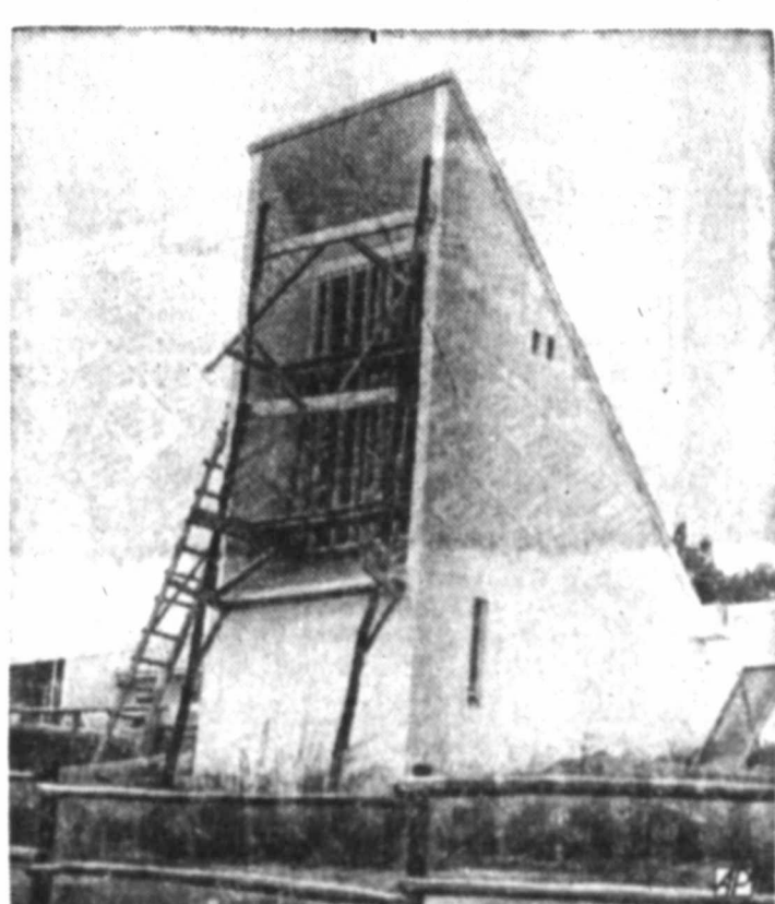
PITCHED ROOF —Chapel of unusual design nearing completion at Mbabane, Swaziland, accommodates tall, stained glass windows by means of a severely slanted roof.
