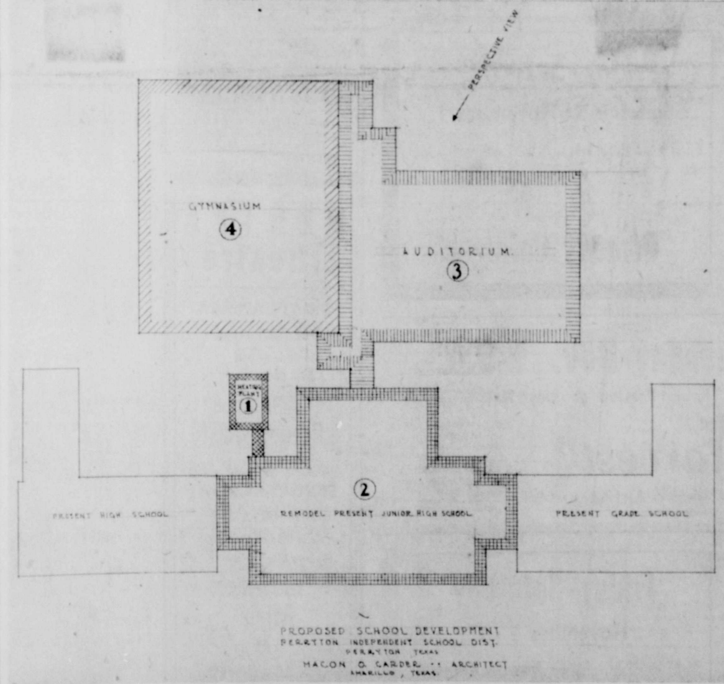
PROPOSED SCHOOL DEVELOPMENT—This view shows how the school plant would look with the addition of the new auditorium, gymnasium and heating-plant. As shown, the gym and auditorium would be located just back of the present center building, connected by an archway. The heating plant (1) would be a separate building, with new equipment capable of heating the whole school plant, including the gym and auditorium. The present center building (2) would be remodeled, making the auditorium into classrooms and would house the junior high school. The auditorium (3) would have a seating capacity of 1,400, making it capable of serving as a community gathering place as well as for all school purposes. The gymnasium (4) would seat 1,500 and allow ample space for both boys and girls physical education classes.
