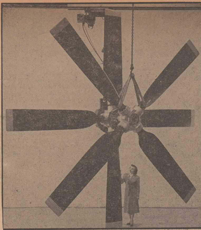
LITTLE GIRL, GAY BLADE —Eighteen feet in diameter, this sprawling "octoprop" makes a midget of the girl standing beside its lower blade. The prop is one of the largest turbo-electric aircraft propellers made today. Eight blades, made of hollow steel, using dual rotation, it is capable of harnessing 15,000 horsepower. Intended for use with a new turbo-prop engine, the octoprop was developed by Curtiss-Wright and the U. S. Air Force.
