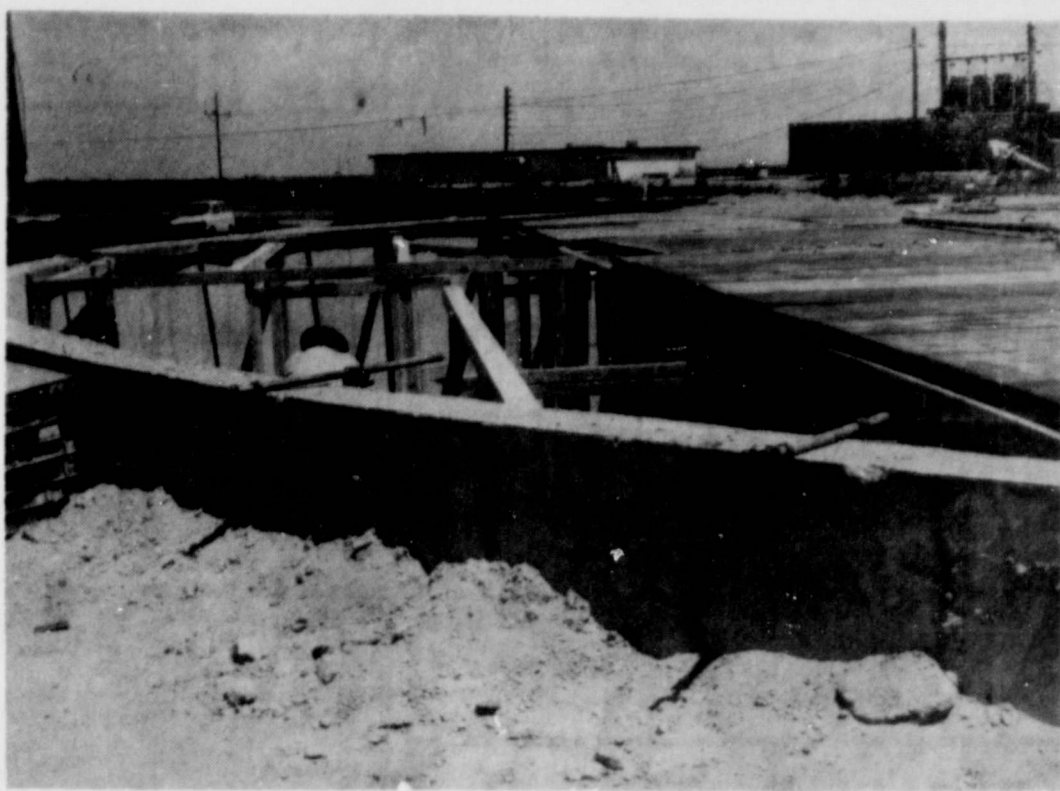
PREPARING FINAL FORMS - The framework for the final forms to be built before all the concrete is poured at the new water reservoir can be seen here. The storage tank will
