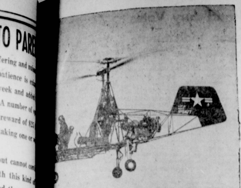
TURBINE POWERED HELICOPTER —The first such gas turbine shaft powered helicopter has been announced. It is the experimental K-225. Although similar in principle to the experimental K-225, the K-225 differs in the application of power jet exhaust gases for direct thrust, the power of the shaft of the rotor blades. (Official Navy photo released for the press.)
