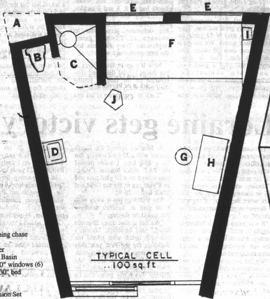
CELL FLOOR PLAN
