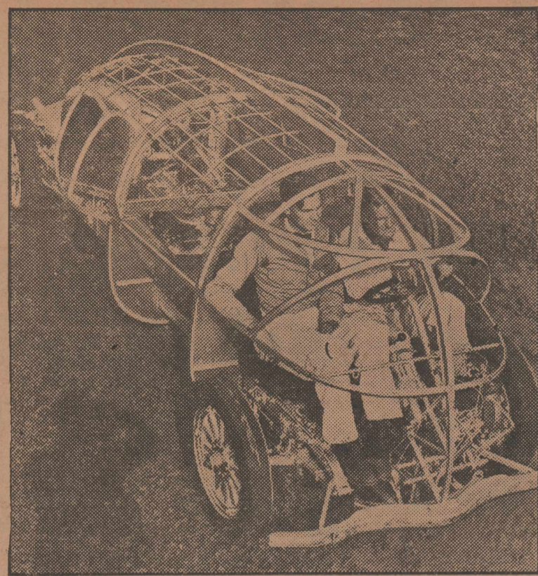
In the car of tomorrow, it seems, the engine will be missing from its usual place. A skeletonized model of a new type automobile, non capsizable, streamlined, and carrying the engine in the rear, is shown as displayed in Hollywood by its inventors, Allen M. Hoppe and Allen F. Streut. There are no running boards and fenders, and the auto can hold six passengers.
