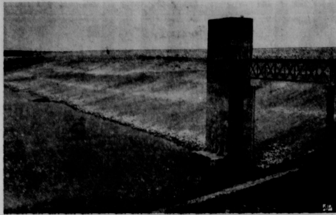
BELTON DAM —This is Belton Dam, a new Central Texas flood control and water conservation project constructed by the U. S. Corps of Engineers and formally dedicated on May 28. Under construction since 1949, the project harnesses the waters of the Leon River, a tributary of the Brazos. The $14,200,000 project consists of a 580-foot long dam, 190 feet high. The dam will form a pool normally covering some 7,400 acres.
