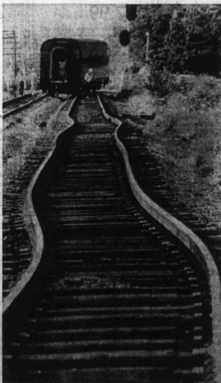
HEAT BUCKLES TRACKS—Extreme heat Sunday caused these railroad tracks near Asbury Park, N.J., to buckle, resulting in the derailment of the passenger car in the background. Temperatures rose into the 90s along Conrail's north Jersey coastline at Spring Lake Heights. (AP Laserphoto)
