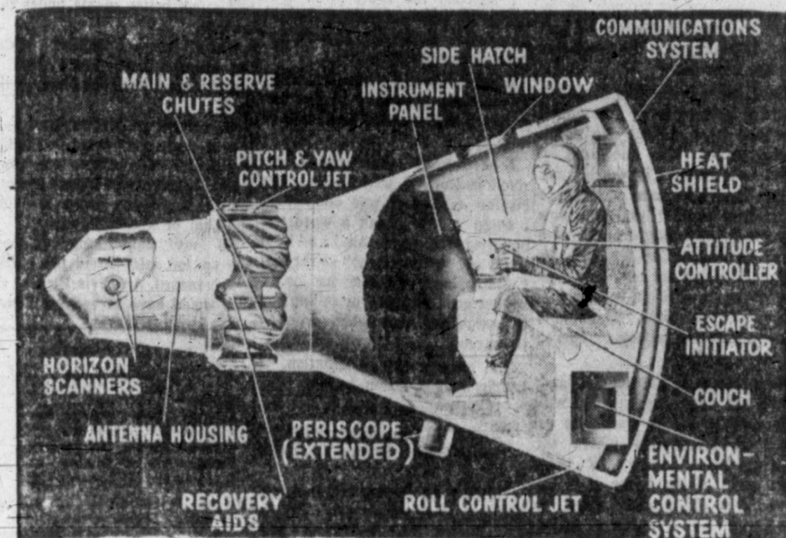
DIAGRAM of Project Mercury's Astronaut Capsule
