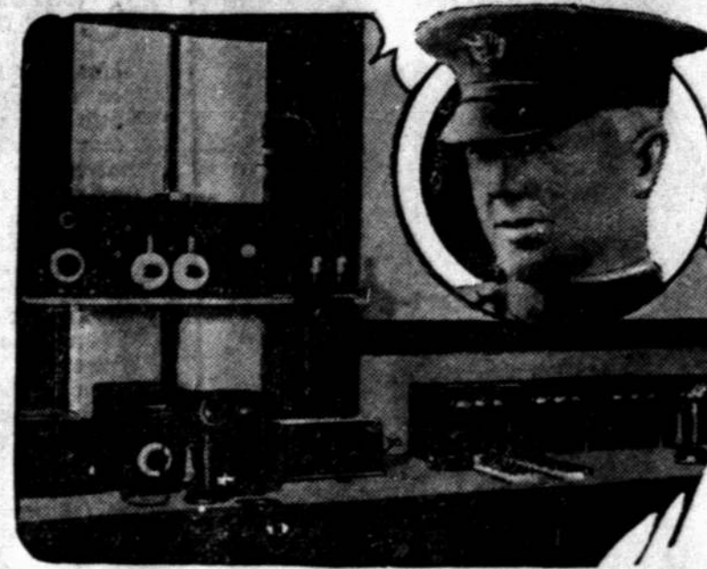
This apparatus is used to carry on two-day wireless telephone conversation between Ft. Leavenworth and Ft. Riley, Kas. Inset shows Capt. C. H. Burkhead, who developed the instruments used.
