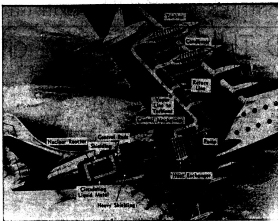
INSIDE AN ATOMIC PLANE... (HOW IT MIGHT LOOK) — This phantom sketch shows how the world's first atomic-powered plane might be built. It would be a sky giant that would dwarf the B-36. Wide, thin wings that permit great speeds will probably require the flying-boat hull. Huge size is necessary to accommodate the very heavy engine. The world's first atomic-powered plane, ordered by the U. S. Air Force, is now taking shape on the drawing boards at Consolidated Vultee Aircraft, Fort Worth, Tex. Flight-testing is not expected until 1955. (Sketch copyright, 1951, by Popular Science Monthly, from NEA-Acme.)
