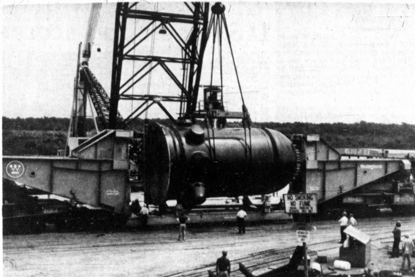
THIS MASSIVE REACTOR vessel for Texas Electric Service Co.'s Comanche Peak nuclear power plant near Glen Rose arrived at the plant site last week. The 347-ton vessel was transported by barge
