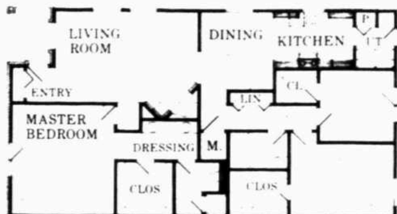
Monterey 1602 Sq. Ft. 3 Bedrooms, 2 Baths
