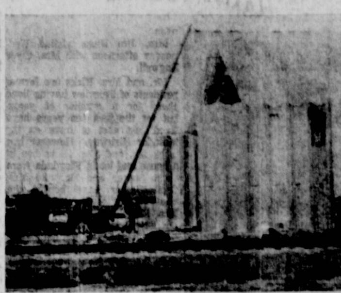
NEW GRAIN STORAGE —Pictured above is the first stages of a new grain storage nearing completion in Floydada. The 50 by 80 structure will house 60,000 bushels of grain, according to Dennis Dempsey, owner. It is being erected by Behlen All Steel Building Corp., of Columbus, Ohio. The crew is from Muleshoe.
