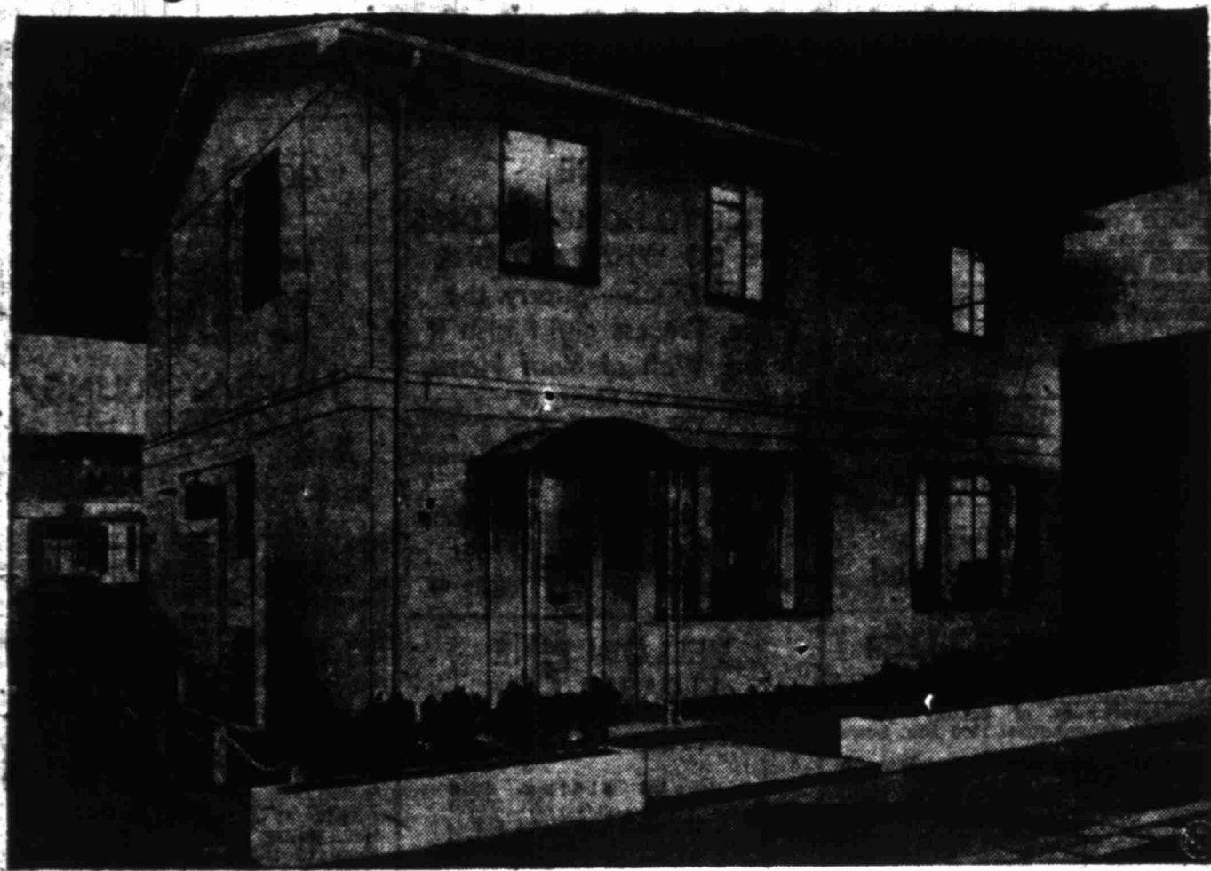
Featured exhibit at London's Ideal Home Exhibition is this two-story pre-fabricated aluminum house. It can be assembled on site in one day. Ground floor sections are built complete in every detail, including equipment, so that site work is limited to bolting them together.
