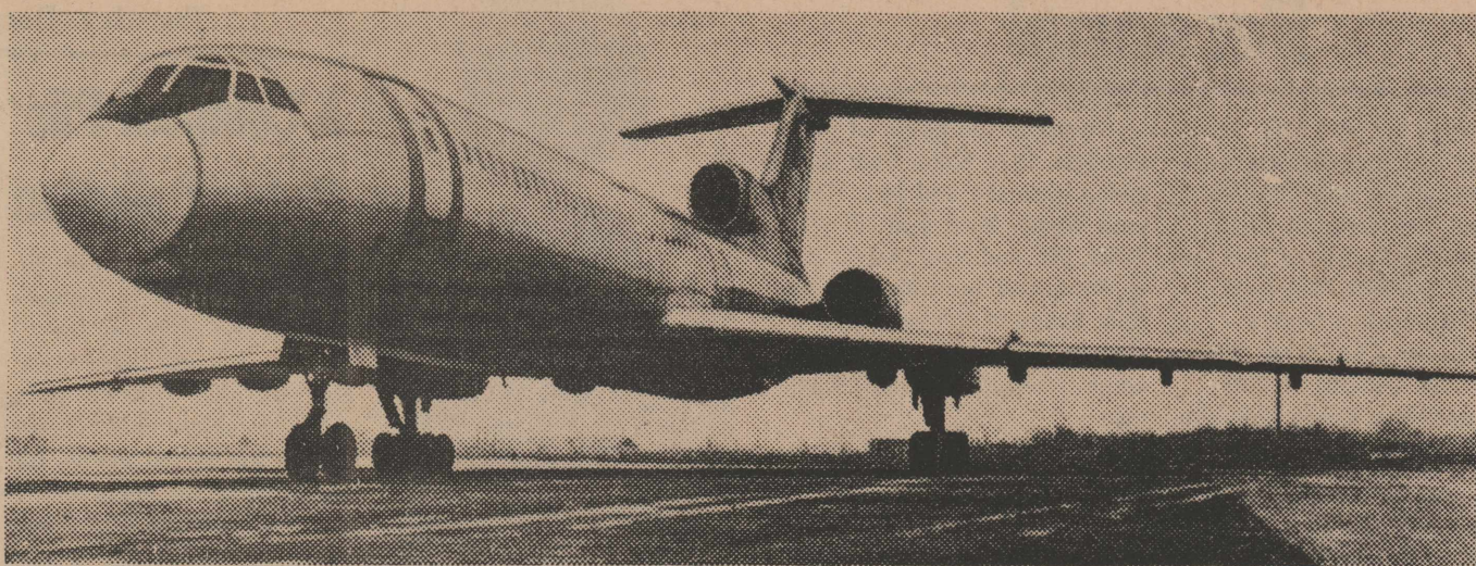
SOVIET SUPERJET is Moscow's answer to the American 747 Jumbo Jet. The TU-154 on a tryout at the Kulbyshev aircraft plant is 164 feet long, has a wingspan of 121 feet and can carry up to 250 passengers. Three tail-assembly jets give it a 590-m.p.h. cruising speed. After tests are completed, the plane will go into service on domestic and international routes of Aeroflot, the Soviet airline.
