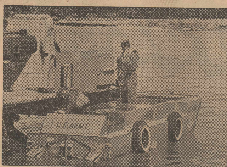
THE SKYLARC, amphibian experimental vehicle, being prepared for its part in the demonstration before the Army Scientific Advisory Panel, held recently at Ft. Eustis, Va. SKYLARC is a research "test bed", embodying desirable features which are being studied for possible use in future Army amphibians. It was constructed by Ingersol-Kalamazoo Division of Borg-Warner Corporation.
