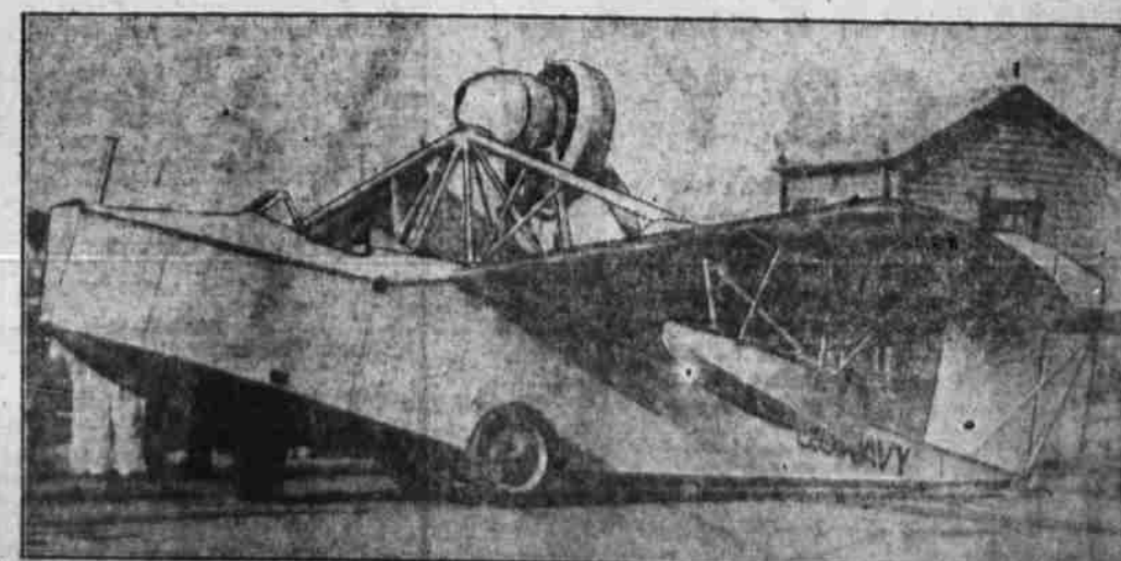
This new small "mystery plane" shown as it was being tested by the United States navy at New York is constructed so that it can be folded in three minutes and dropped into an eight foot torpedo tube on submarines. Powered with a 110-horsepower radial engine, the plane reached a speed of 100 miles an hour.
