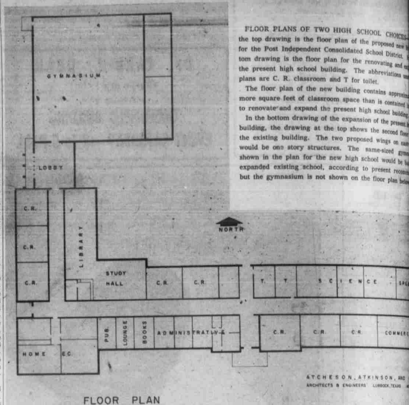
FLOOR PLAN
