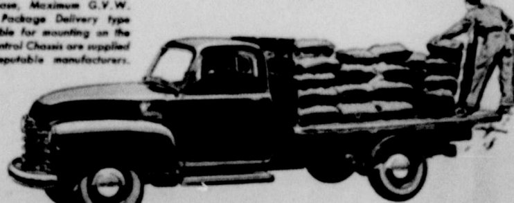
MEDIUM-DUTY CAB AND CHASSIS WITH PLATFORM BODY Model 3000—137 inch wheelbase, Maximum G.V.W. 8,800 lb. Other models available up to 161 inch wheelbase and 16,000 lb. G.V.W.
