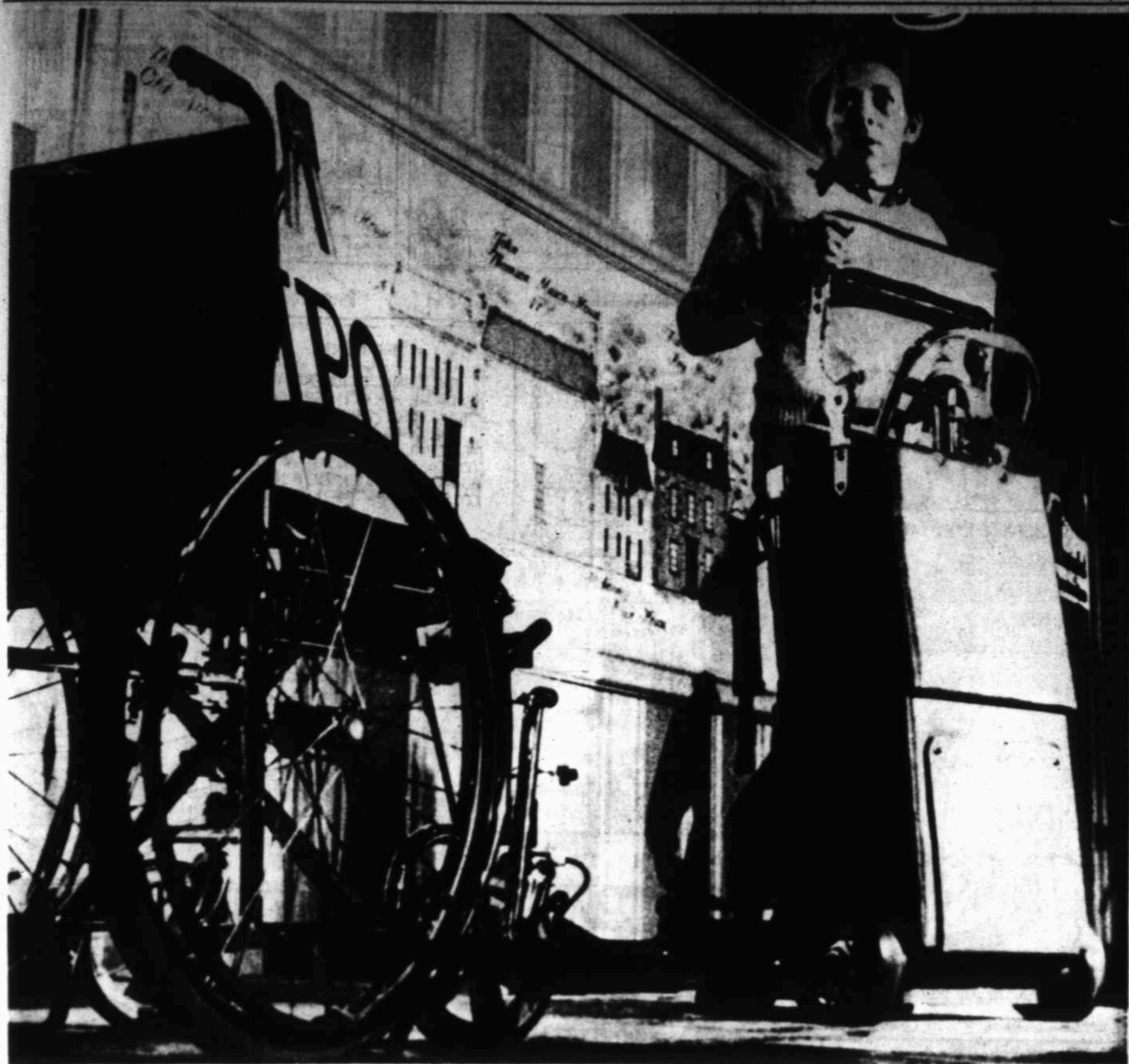
Donald Ausmus, a 40-year-old paraplegic from Independence, Mo., demonstrates his invention of the Moto-Stand, a battery-driven device that allows physically handicapped
