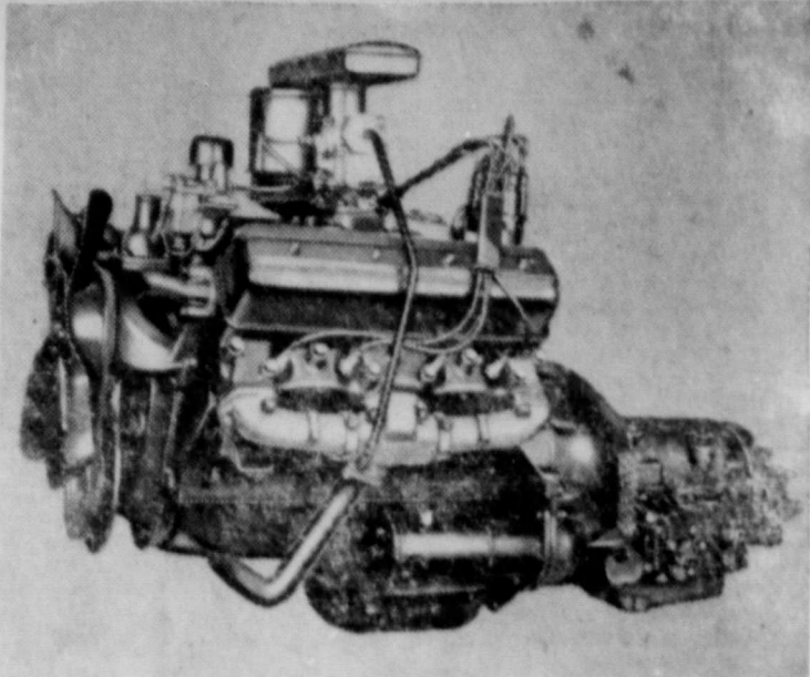
Side view of Studebaker's new 8-cylinder, valve-in-head engine which powers the 1951 Commander series. Rated horsepower of the new V-8 engine is 120 at 4000 r.p.m. Taxable displacement is 232.6 cu. in. Bore and stroke, 3 1/4" x 4 1/4", respectively. Compression ratio as released.
