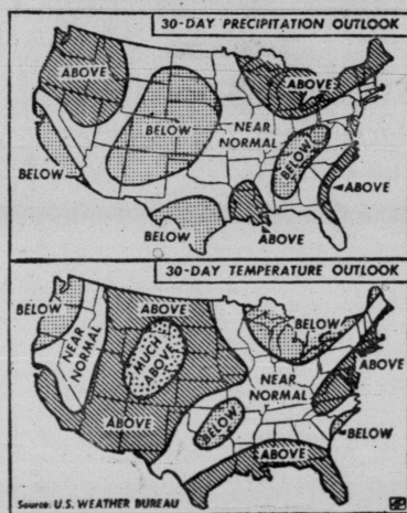
WEATHER FORECAST FOR NEXT 30 DAYS — These maps, based on those supplied by the United States Weather Bureau, forecast the probable rainfall and temperatures for the next 30 days. (AP Wirephoto Map)
