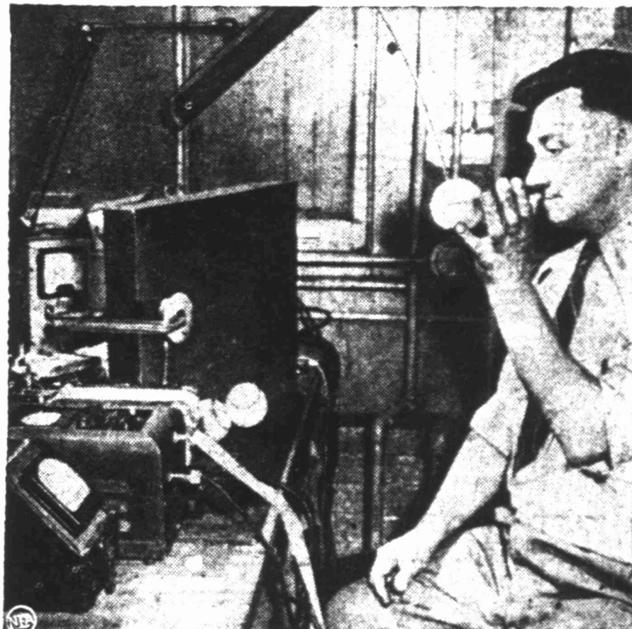
TRY THE BATS! —Service Engineer John Halter of a Cleveland development company bounces a suspended American League baseball against a metal plate, with the vibrations being recorded automatically. The company's scientists found no rabbit in the 1930 horsehide, concluding that there was "no measurable difference" between the 1949 and '50 major league balls.
