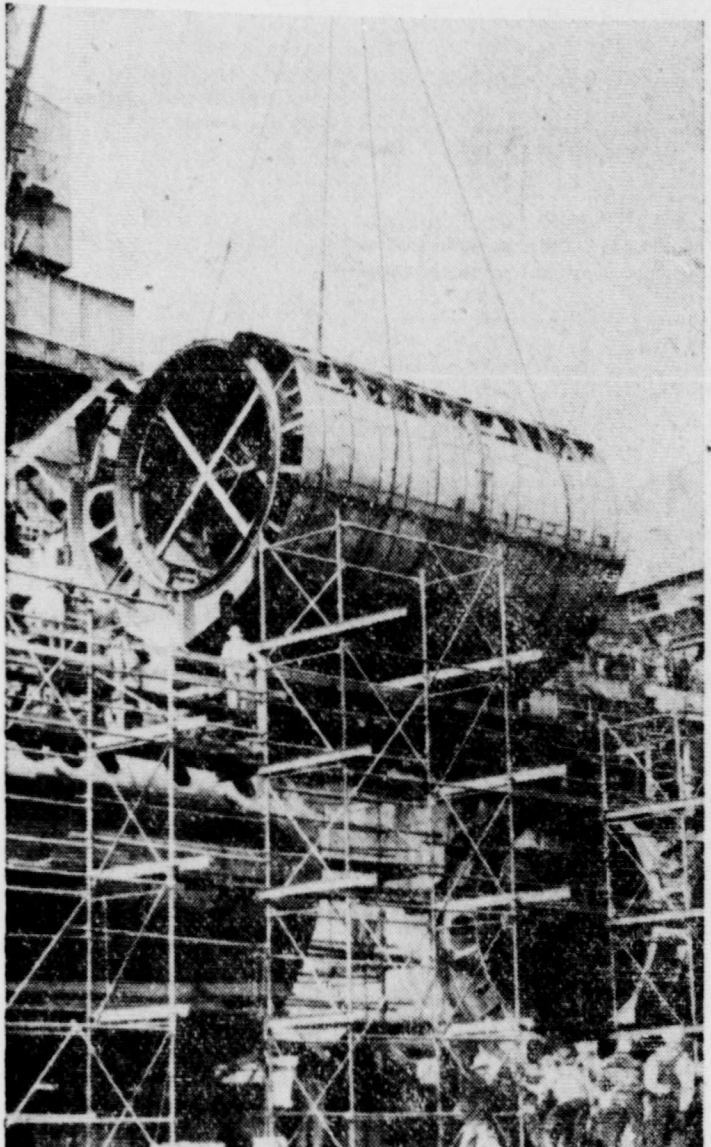
CHEAP AT THE PRICE —At the Naval Base in Philadelphia, Pa., a crane is lowering a 60-ton, 30-foot-long, prefabricated section between the two divided parts of the submarine Raton. The cost of enlarging the sub is estimated at $6,000,000 as against a cost of between $15,000,000 and $20,000,000 to build an entirely new craft of similar design.
