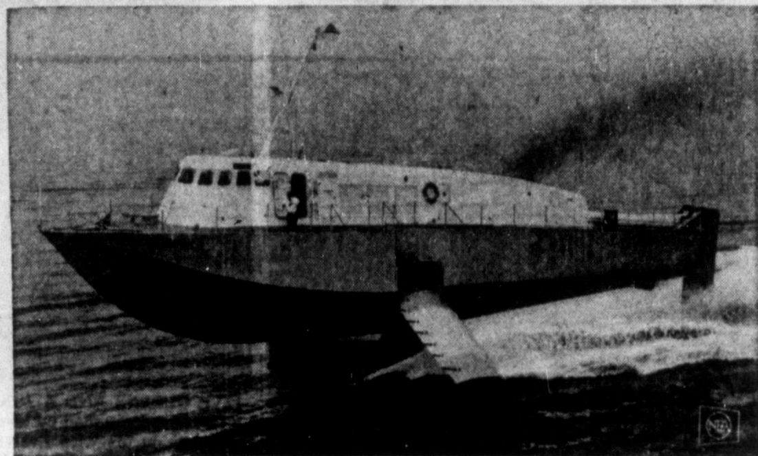
HIGH-STEPPER—The HS (Hydrofoil Ship) Denison is shown making its first "flight" in Long Island Sound. Raised up on its underwater wings, the 90-ton craft reached a speed of 50 knots. Developed by Grumman Aircraft, the 104-foot-long aluminum vessel is expected to be the first operational, ocean-going hydrofoil ship. The Denison will be employed as a passenger ship in 1963 along a tourist route between Florida and the Bahamas.
