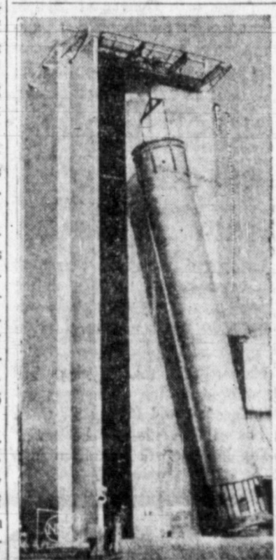
TOWER TEST —A 105-inch diameter, 62-foot-high liquid oxygen tank for the Saturn rocket is removed from tower at Dallas, Tex., after it was water-tested for leaks.
